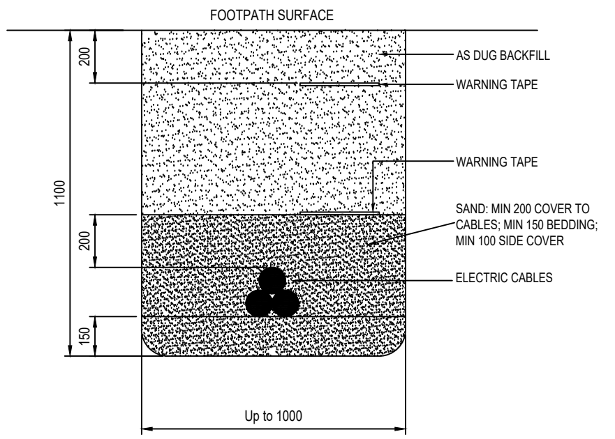
TYPICAL CABLE TRENCH DETAIL SCALE 1:20
